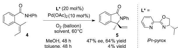
Scheme 1. Initial experiments to explore the catalytic reaction.
