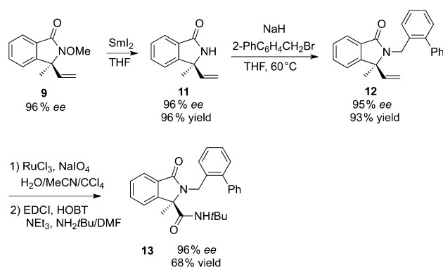
Scheme 3. Further transformation of an isoindolinone product. EDCI = 1-(3-dimethylaminopropyl)-3-ethyl-carbodiimide, HOBT = 1-hydroxybenzotriazole.
