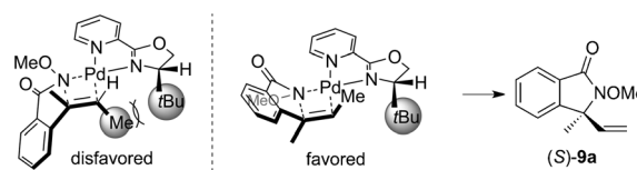
Scheme 2. Model for explaining the origin of asymmetric induction.
