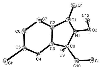
Figure 2. ORTEP representation of 9j ; thermal ellipsoids are shown at 30 % probability and hydrogen atoms are omitted for clarity.
