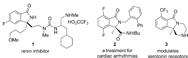
Figure 1. Representative examples of isoindolinones bearing tetrasubstituted carbon stereocenters \alpha to the nitrogen atom.
